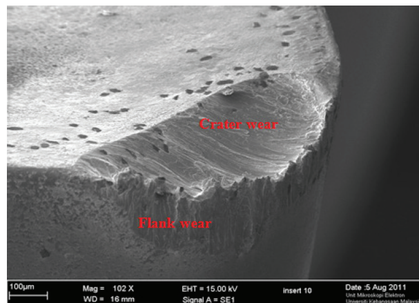
FIGURE 4. SEM micrograph (scale 100 \mu\text{m} ) shows the flank and crater wear on CNGG 120408-SGF-H13A
